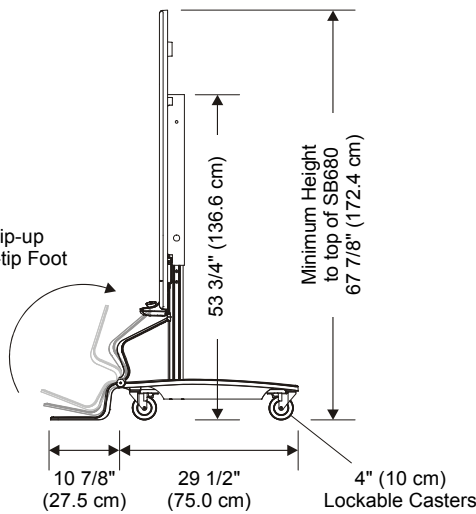
Floor Stand Mounted Side View (lowest position)
