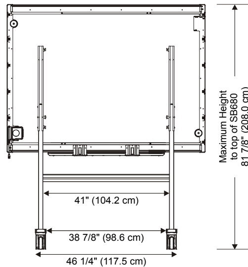
Floor Stand Mounted Back View (highest position)
