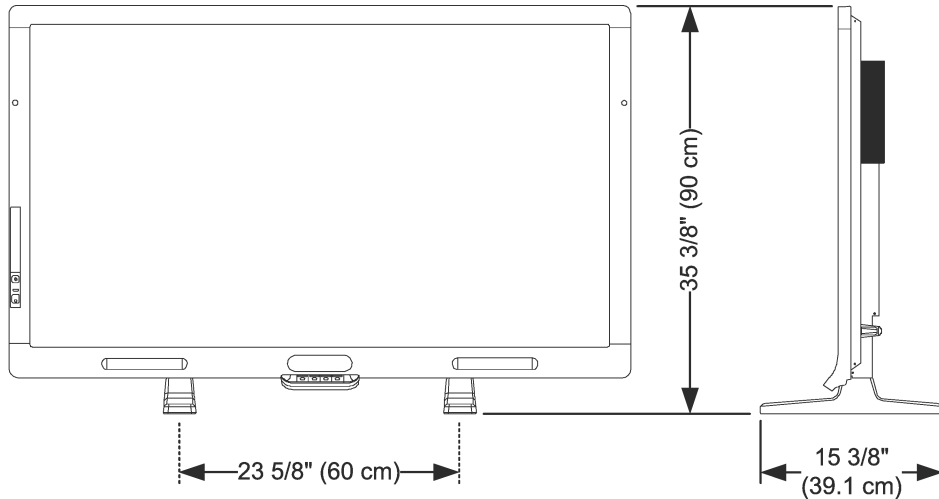
Front and side view with interactive flat panel
