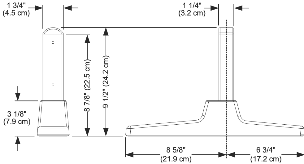
Front and side view
